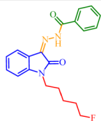
5F-BZO-POXIZID
